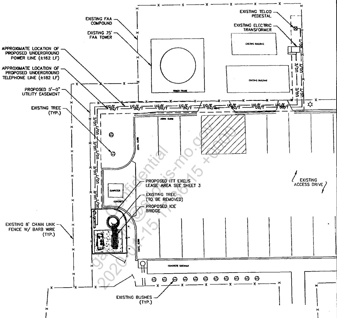
SITE PLAN
