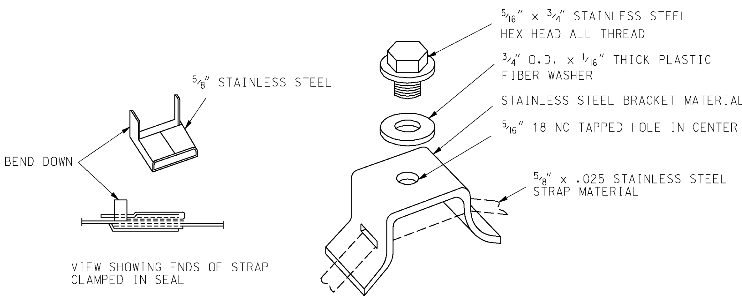
STRAP SEAL FLARED LEG SIGN BRACKET
