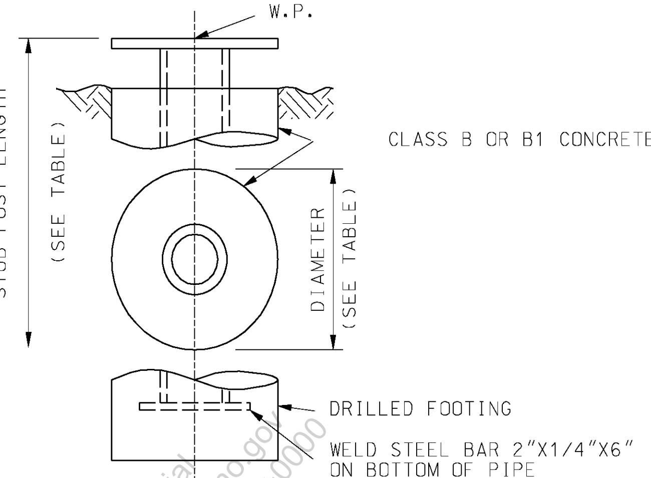
SLIP BASE ASSEMBLIES FOUNDATION DETAIL
