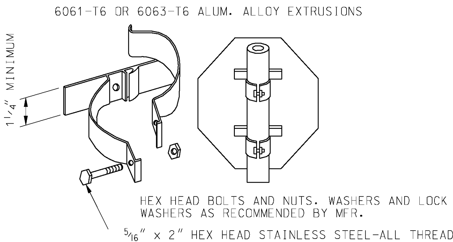
CLAMP TYPE SIGN SUPPORTS FOR PIPE POST
