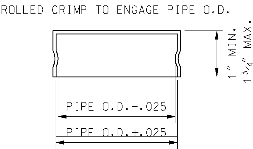
FRICTION CAP
