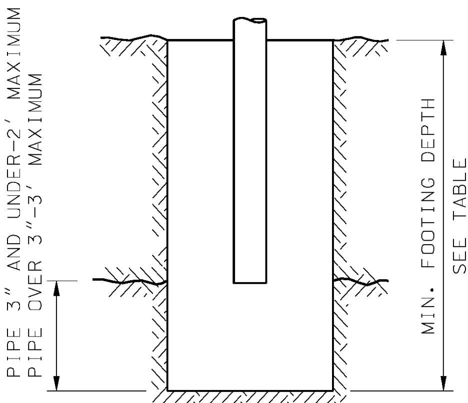
FOOTING IN ROCK
