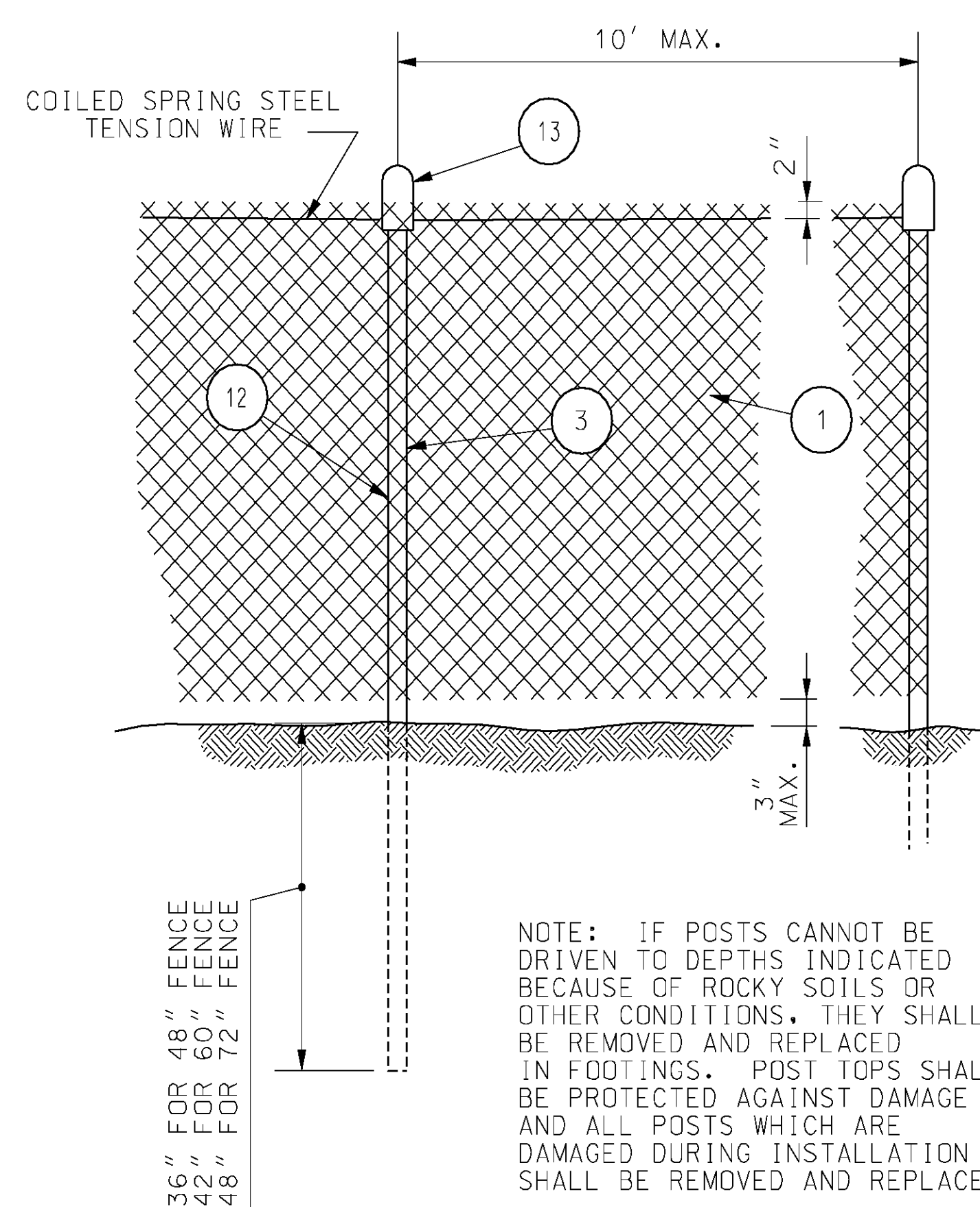
ALTERNATE LINE POST ANCHORAGE (DRIVEN)
