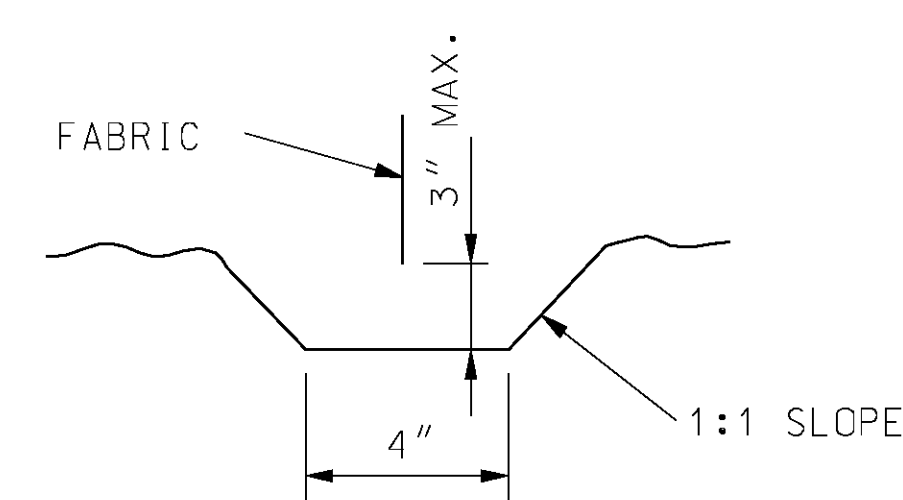
TYPICAL TRENCH DETAILS
