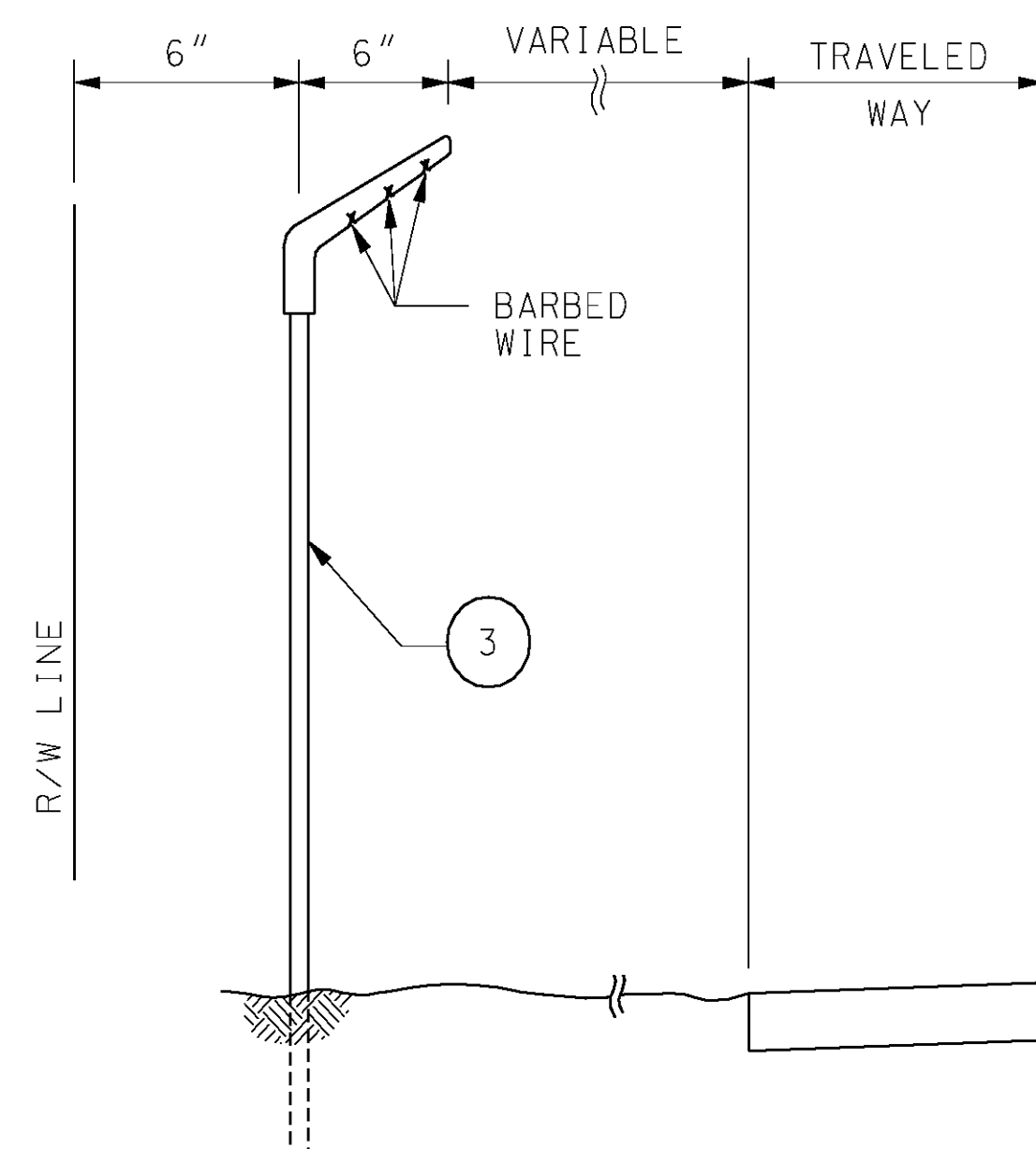
BARBED WIRE EXTENSION BRACKET
