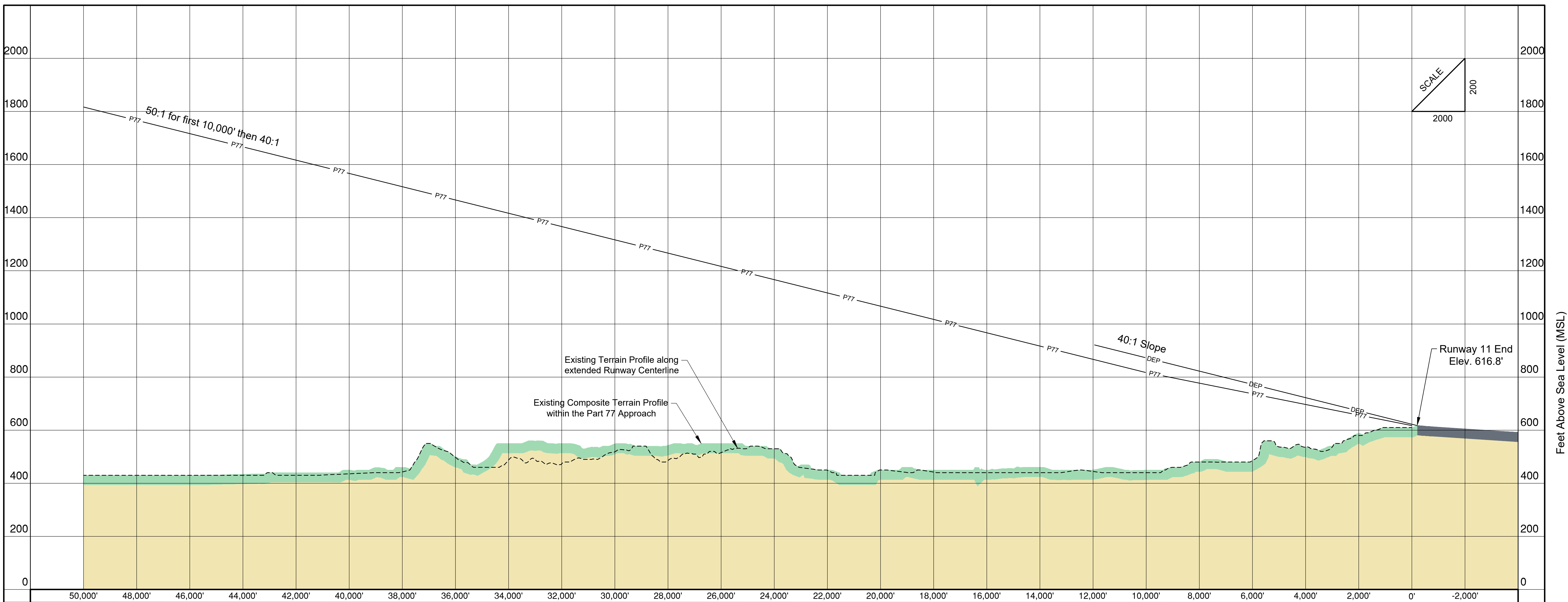
Runway 11 Profile View Scale 1"=2000' Horizontal 1"=200' Vertical
