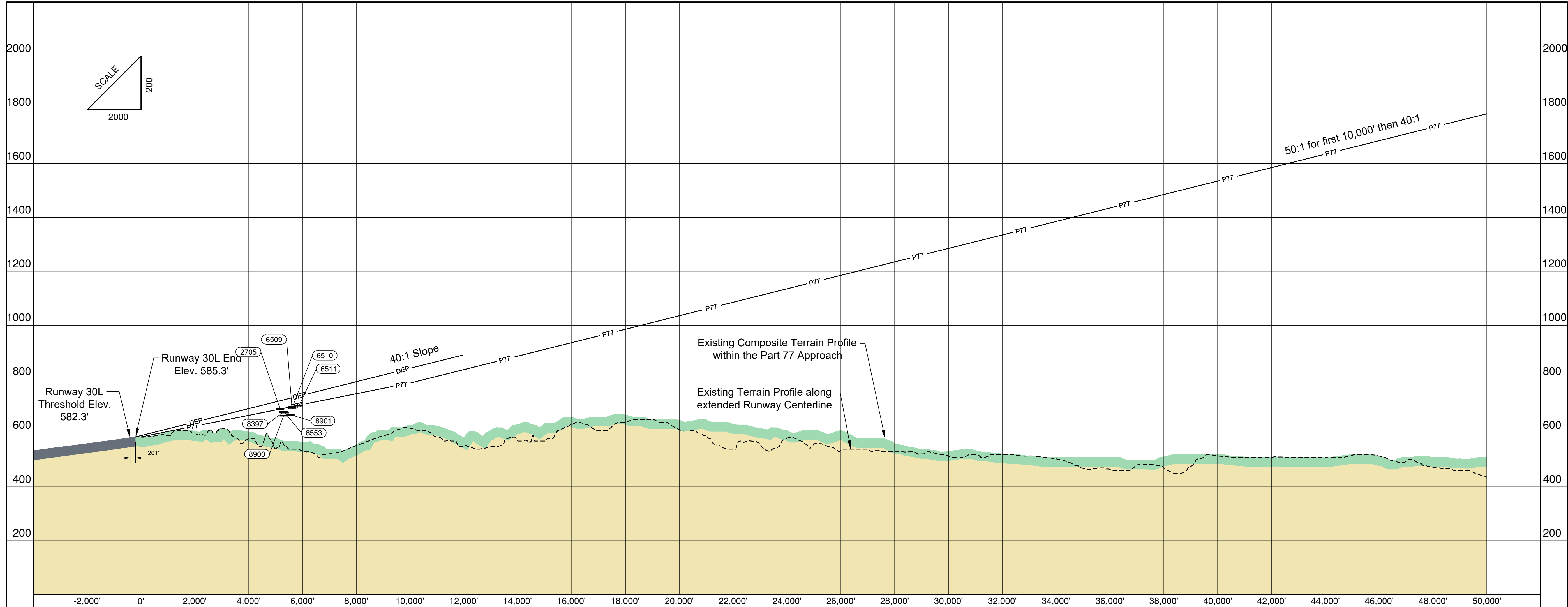
Runway 30L Profile View Scale 1"=2000' Horizontal 1"=200' Vertical
