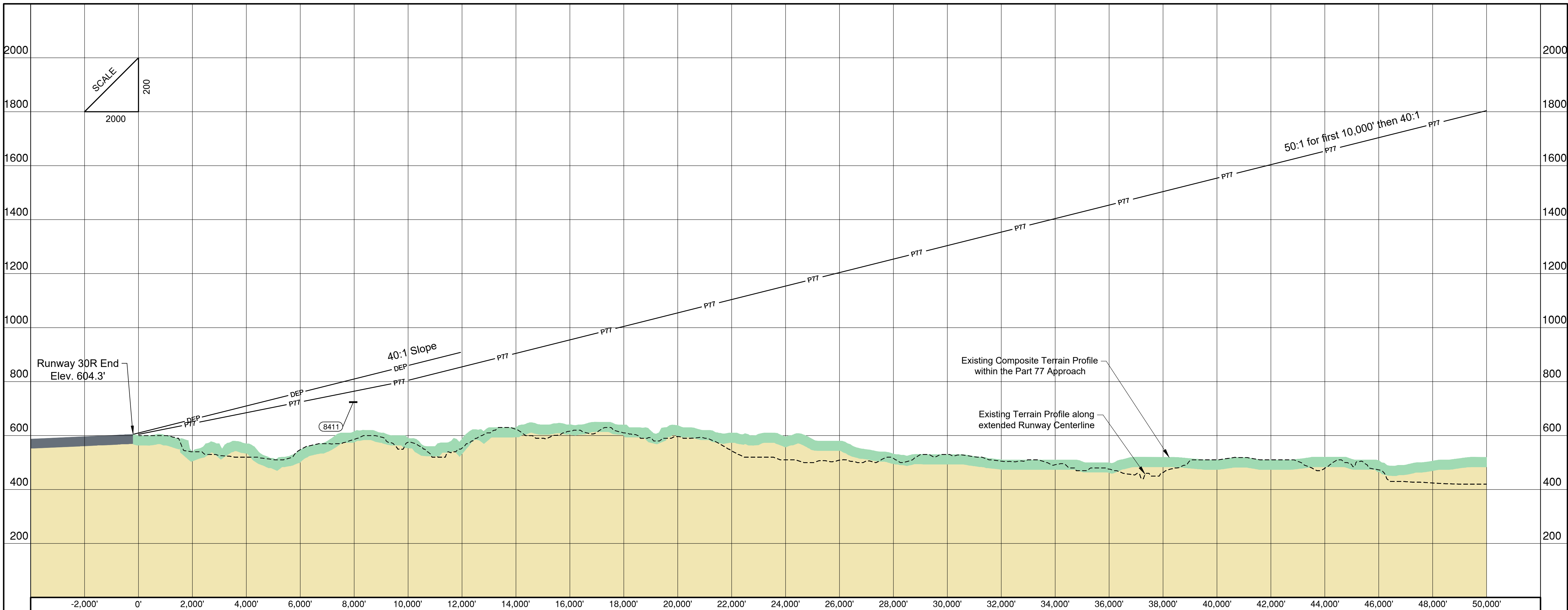
Runway 30R Profile View Scale 1"=2000' Horizontal 1"=200' Vertical
