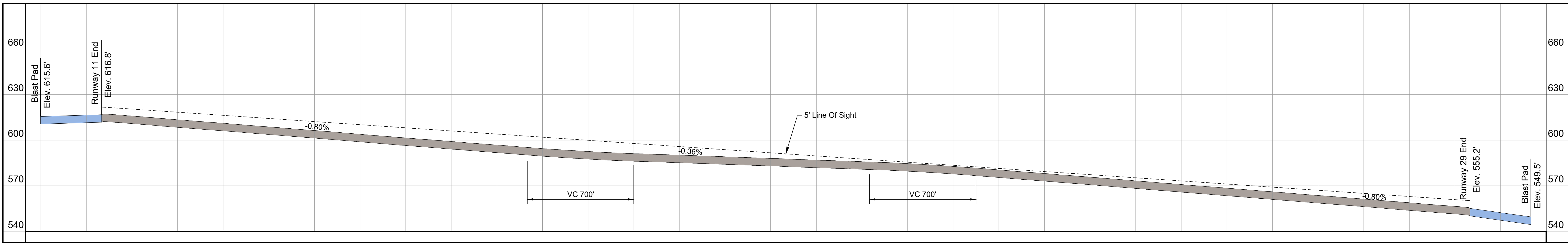
Runway 11/29 Profile View (Existing)
